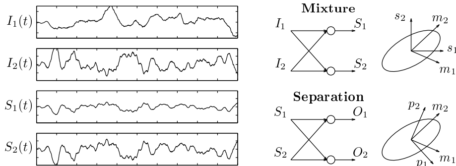
Figure 1: Mixture of sources and blind separation.
