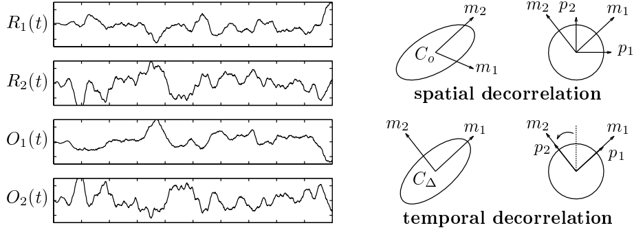
Figure 2: Spatial and temporal decorrelation.
