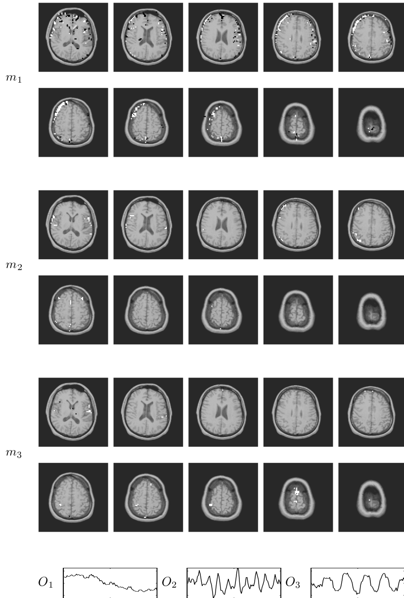
Figure 6: fMRI activity patterns during simple flexion performed with the left hand of a subject. Shown on the top are the leading three activity patterns m_1 , m_2 , and m_3 , for which the corresponding temporal traces O_1 , O_2 , and O_3 are shown at the bottom (the same as the leading ones in Fig. 5). They account for 17.7%, 4.7%, and 4.4% of the signal variance.
