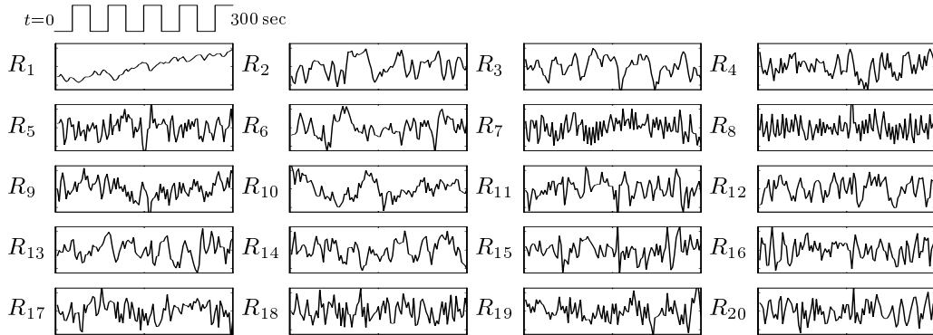
Figure 4: Spatial decorrelation. Shown in the figure are the top 20 temporal traces which are decorrelated spatially. The vertical zero is at the middle of each plot. The scale of the vertical axis is not marked, since only the relative amplitude and the relative sign are meaningful.
