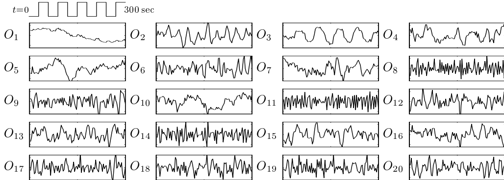
Figure 5: Temporal decorrelation. Shown in the figure are the top 20 temporal traces which are decorrelated spatially and temporally. The vertical zero is at the middle of each plot with upward for positive and downward for negative (see the text for the sign convention). For the top three temporal traces O_1 , O_2 , and O_3 , the corresponding activity patterns are shown in Fig. 6.
