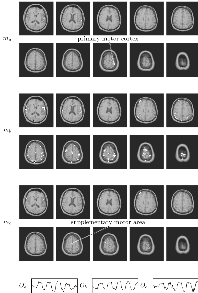
Figure 7: fMRI activity patterns for three different ways of finger tapping performed with the right hand of a subject. They are (a) simple flexion, (b) sensorimotor sequences, and (c) imagining sensorimotor sequences. Shown on the top are the three task-related activity patterns m_a , m_b , and m_c , for which the corresponding temporal traces O_a , O_b , and O_c are shown at the bottom. They account for 3.0%, 12.2%, and 2.2% of the signal variances of the corresponding experiments, respectively.
